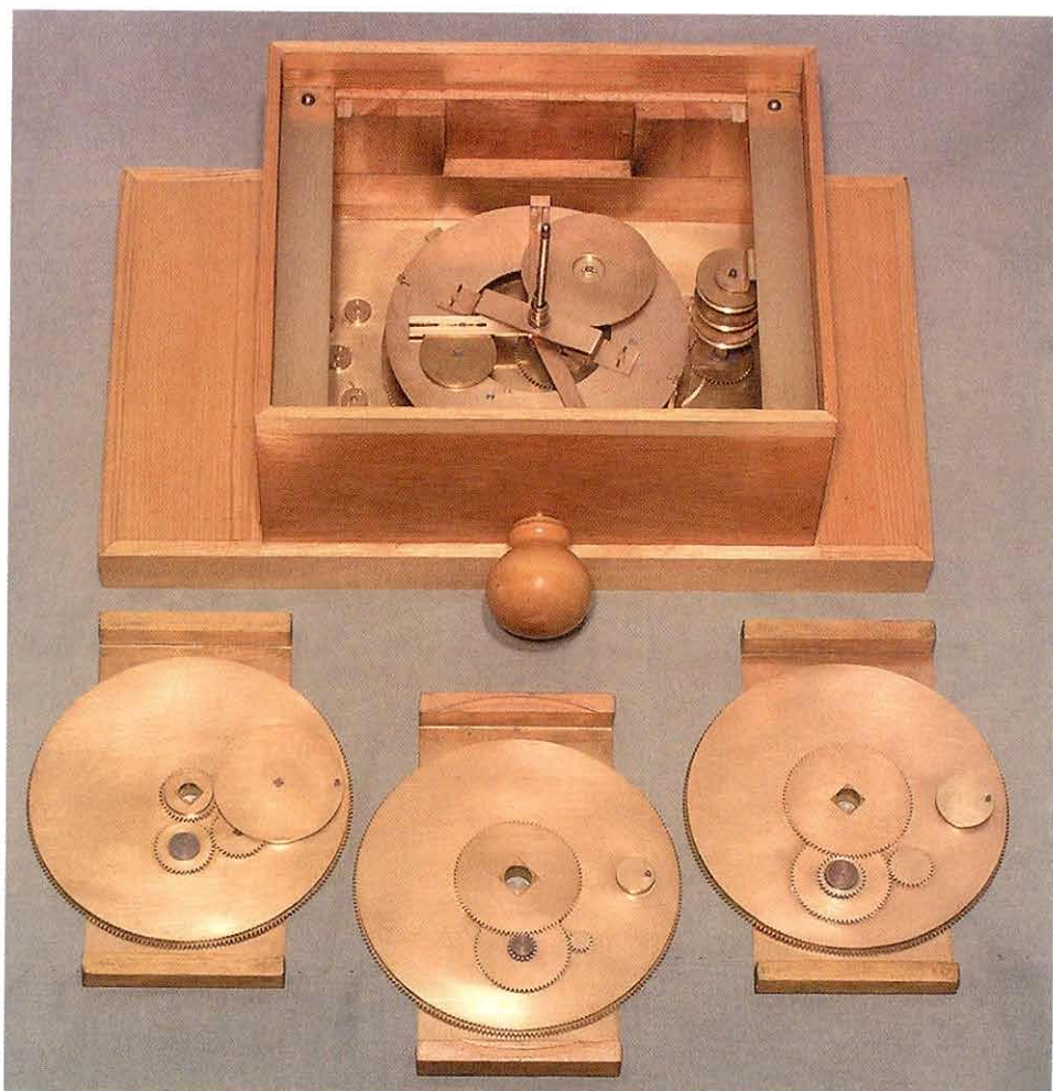
Fig. 7. Model by M.T. Wright, partly disassembled. The gear trains for the Sun, Moon and inferior planets (Mercury and Venus) are in place on the internal frame plate. Conjectural assemblies containing trains for the superior planets (Mars, Jupiter and Saturn), which lie over the frame plate and under the dial, are lifted out.
