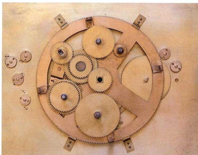
Fig. 4. Model by M.T. Wright, front view of internal frame plate. Compare with figure 3. Note that some screw-fastenings have been used for convenience in place of rivets.
