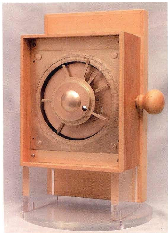
Fig. 1. Reconstruction of the Antikythera Mechanism by M.T. Wright, front view.
