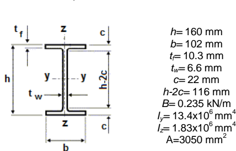
Figure 5: Properties of W150x24 steel section
