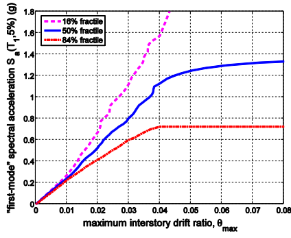
(a) 3ELF 4-story ( SD1_{max} )
