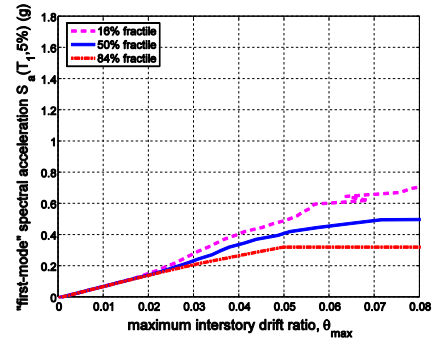
(b) 5ELF 1-story ( SD1_{min} )
